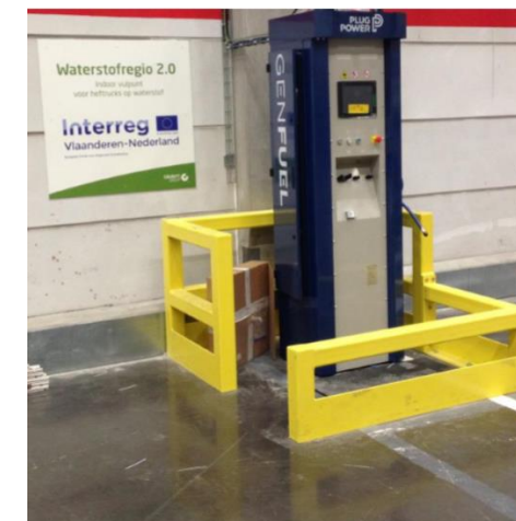
Indoor H2 dispenser Material Handling Vehicles (MHV's)
