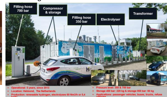
Upgrade H2 station Helmond
